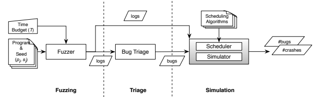
Figure 1: FUZZSIM architecture.
